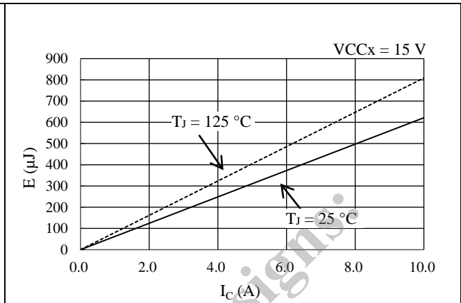
Figure 15-52. Low-side Switching Loss
