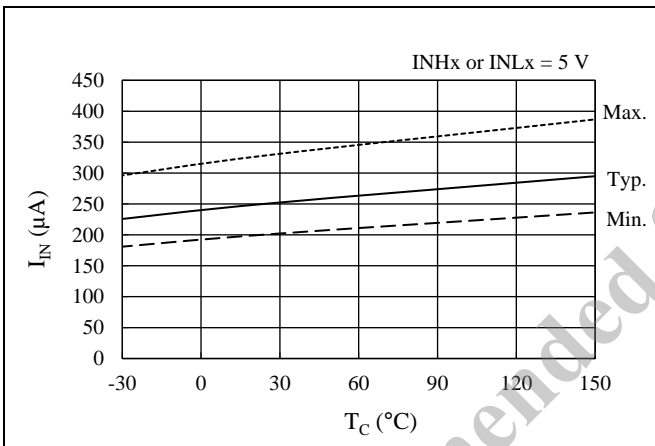
Figure 15-15. Input Current at High Level ( I_{INx} or I_{INLx} ), I_{IN} vs. T_C
