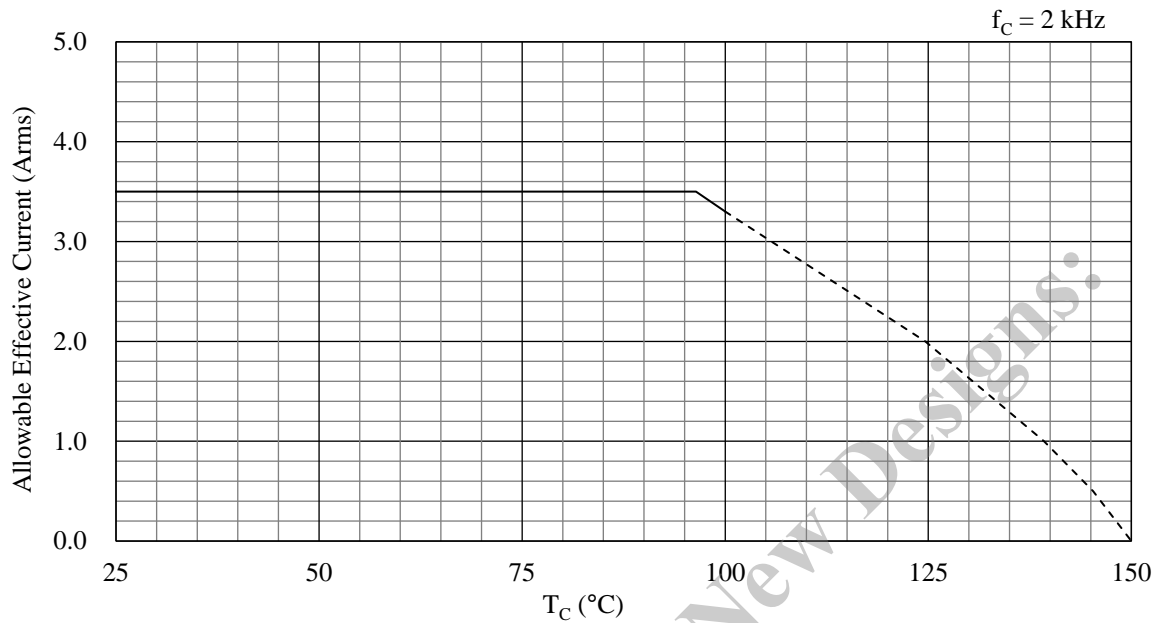
Figure 15-63. Allowable Effective Current (f C = 2 kHz): SIM6895M
