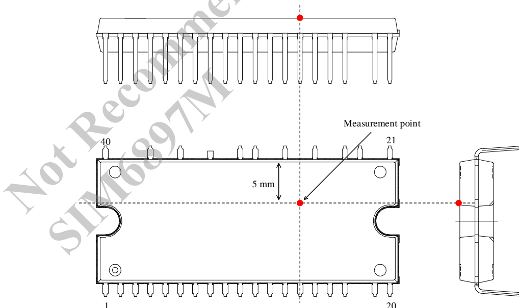
Figure 3-1. Case Temperature Measurement Point
