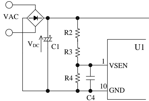
Figure 8-28. VSEN pin peripheral circuit
