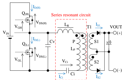
Figure 8-3. Current Resonant Power Supply Circuit
