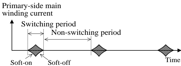
Figure 8-19. Standby waveform
