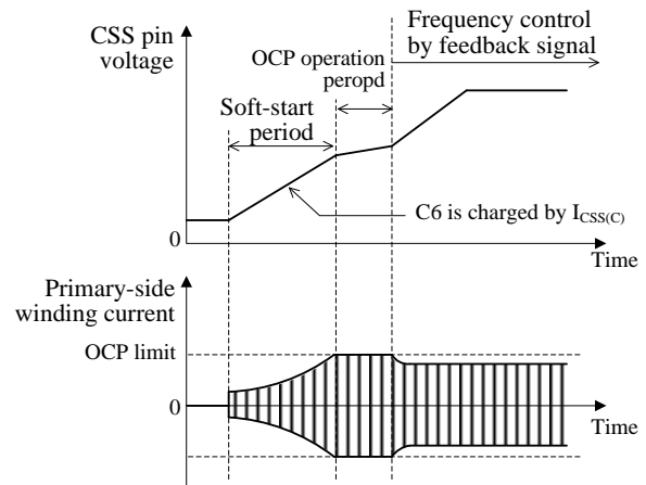
Figure 8-15. Soft-start operation
